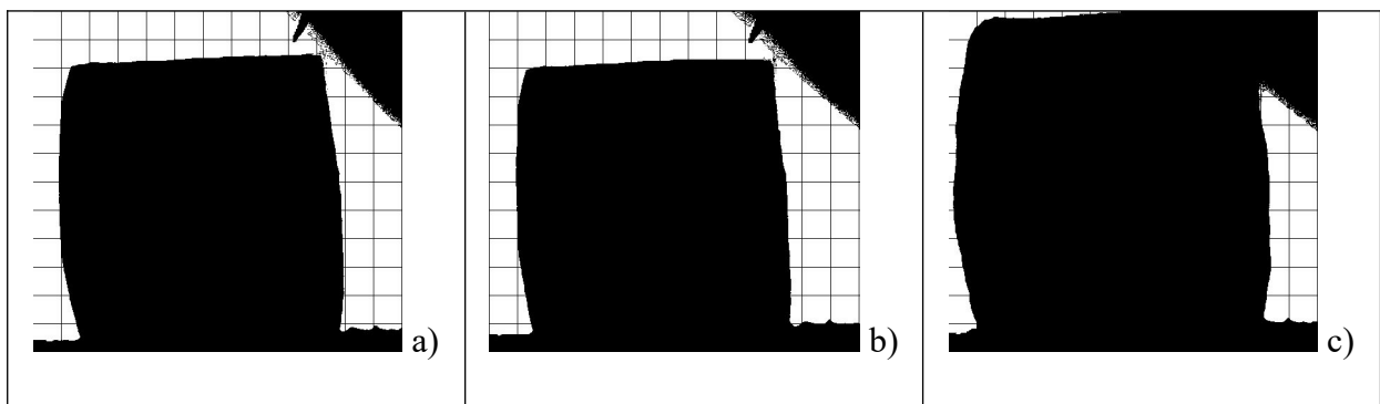
Fig. 7. HSM silhouettes at 30°C (a), 930°C (b) and 980°C (c).
